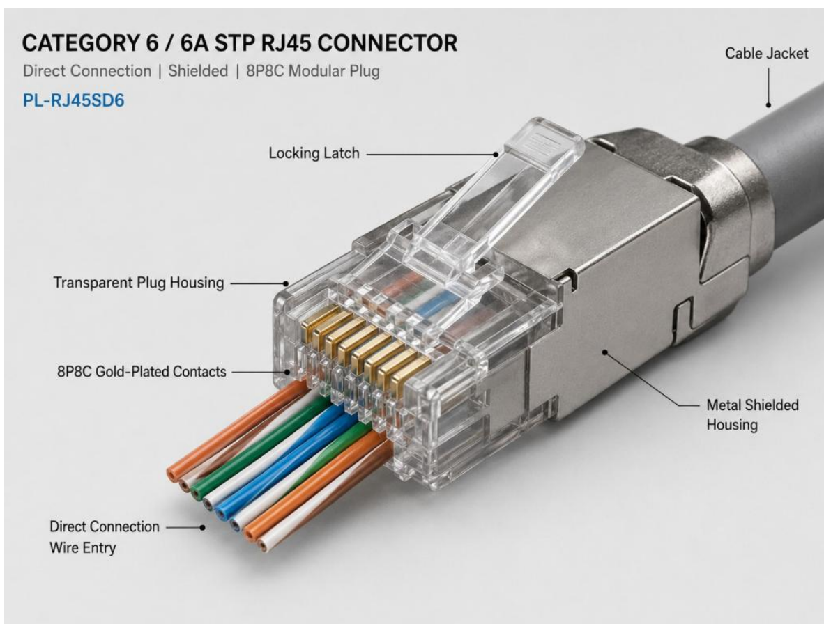
CAT6/6A STP RJ45 Direct Connector - Annotated 3D View
